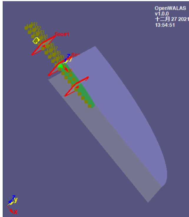
Fig. 6-4 Wigley ship
